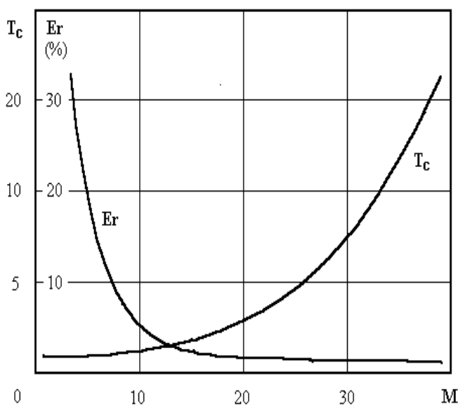
Fig. 2 Computer time T_c in relative units and relative error Er as the functions of the harmonic number M
