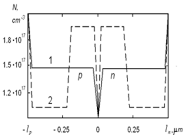
Fig. 1 Doping profile for two types of IMPATT diodes: 1 - constant doping profile; 2 - quasi-Read-type profile
