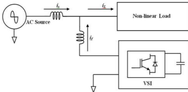
Circuit diagram of shunt active power filter
