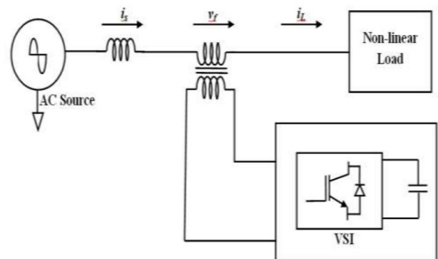
Circuit diagram of series active power filter
