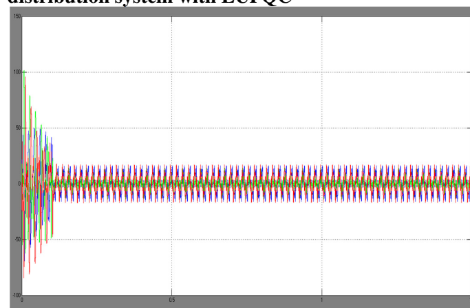
Three phase source current and neutral current distribution system with EUPQC
