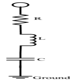
Low pass filter
