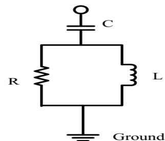
High pass filter
