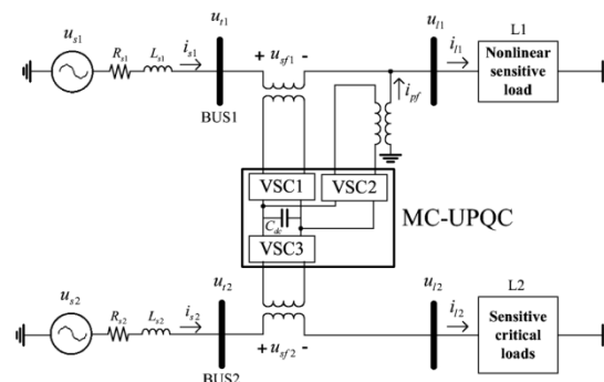
Typical MC-UPQC used in a distribution system.
