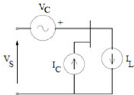
Equivalent circuit of UPQC
