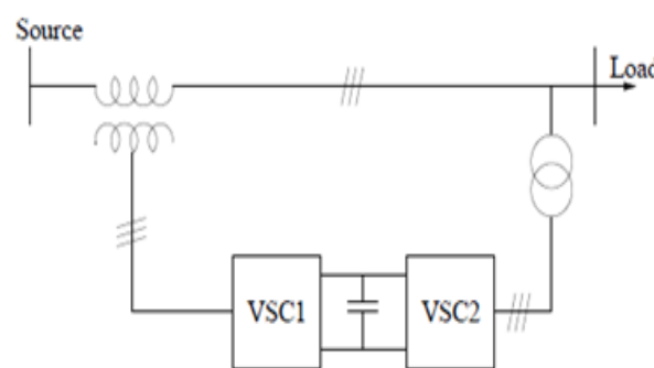
UPQC scheme
