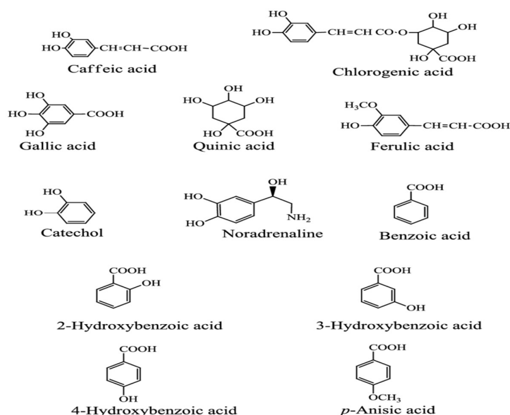
Fig 2: phenolic compounds
