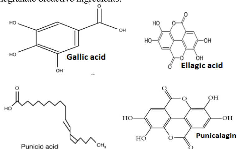
Fig 6: Structure of bioactive compounds obtained from pomegranate
