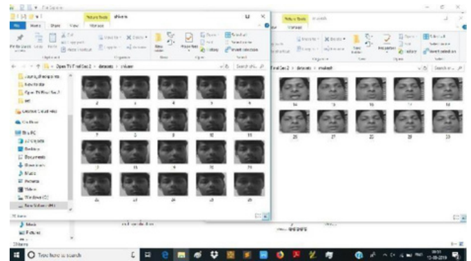
Figure 6: Training Database
