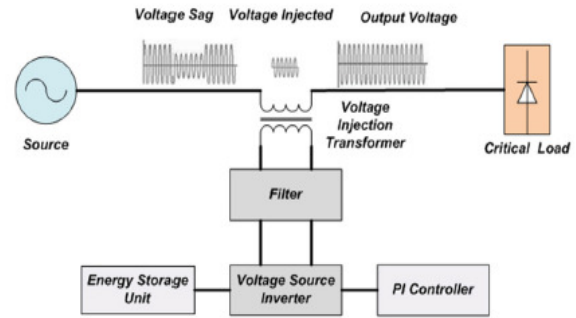
Fig. 3: Basic Proposed DVR
