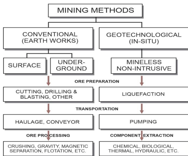
Fig 4. Conventional and GT mineless methods comparison chart.
