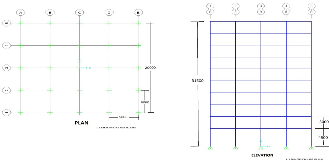
Figure 1: Plan & Elevation
