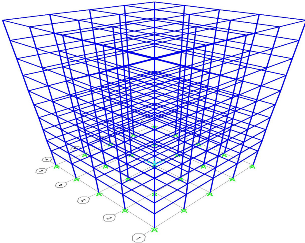
Figure 2 3D View in SAP2000
