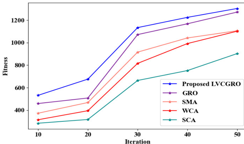
Figure 6: Fitness Vs Iterations
