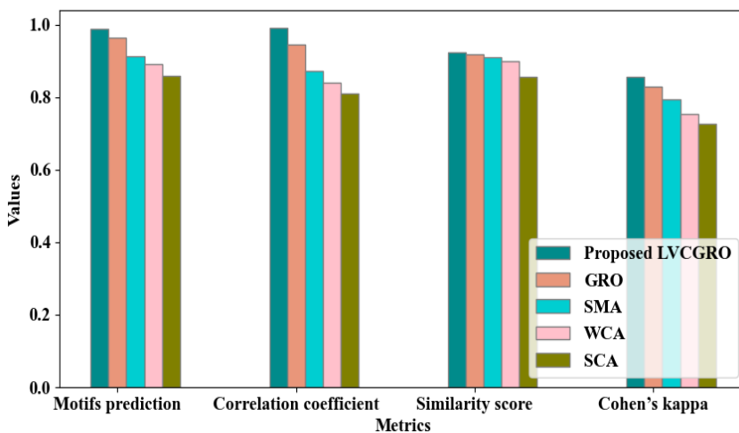
Figure 3: Performance analysis of motif filtering
