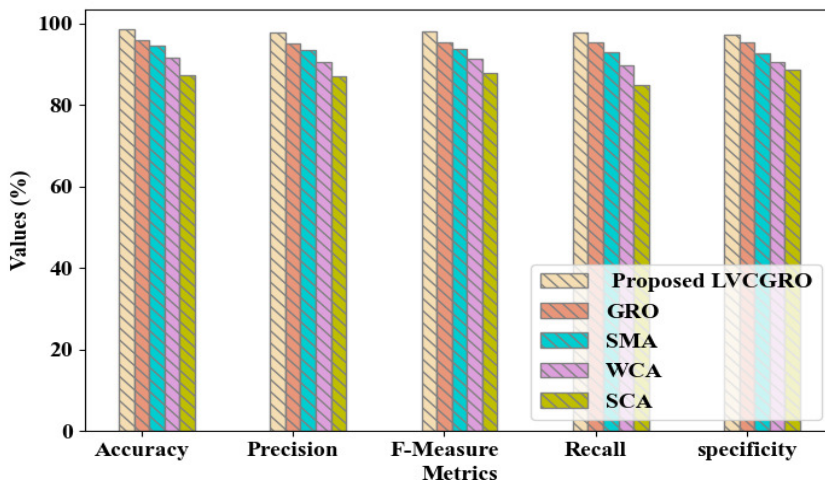
Figure 2: Performance Comparison of proposed LVCGR0
