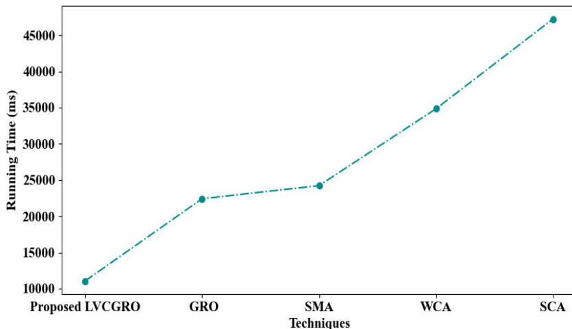
Figure 4: Running Time Analysis
