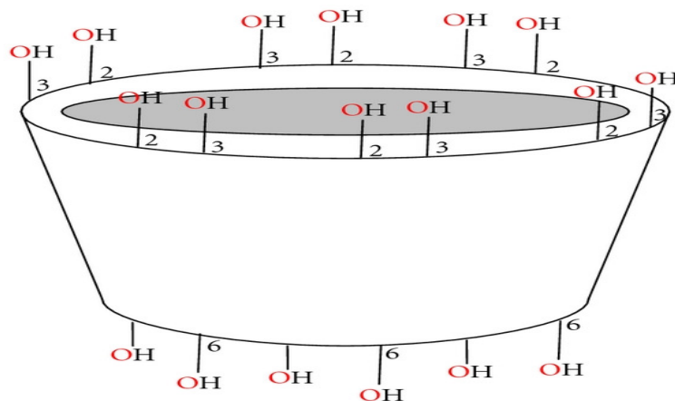
Fig 1: Representations of hydrophobic cavity and hydrophilic outer surface of cyclodextrin.
