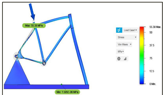
Figure 14. Stress simulation of bike frame and support
