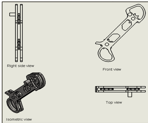
Figure 5. Variator and its views
