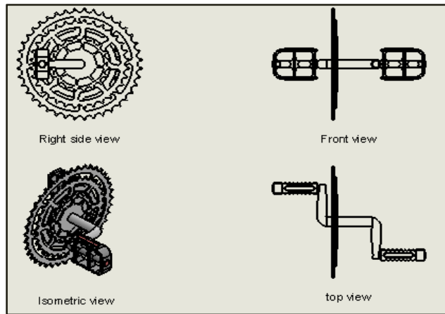
Figure 3. Sprocket with pedal link and its views
