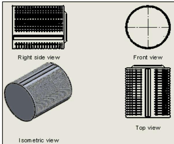
Figure 8. Inner drum and its views
