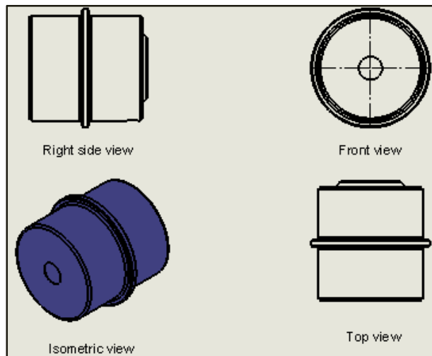
Figure 9. Outer drum and its views
