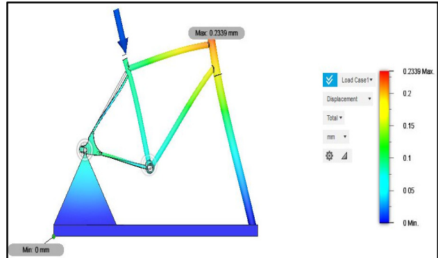
Figure 12. Displacement simulation of bike frame and support
