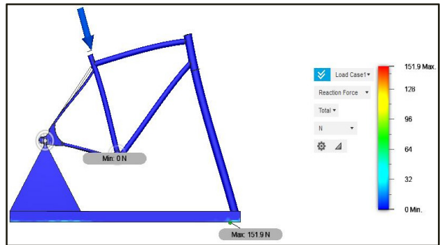
Figure 13. Reaction force simulation of bike frame and support
