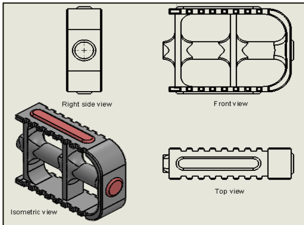
Figure 2. Pedal and its views
