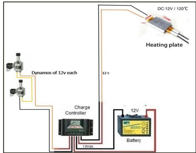
Figure 10. Electrical part of the model
