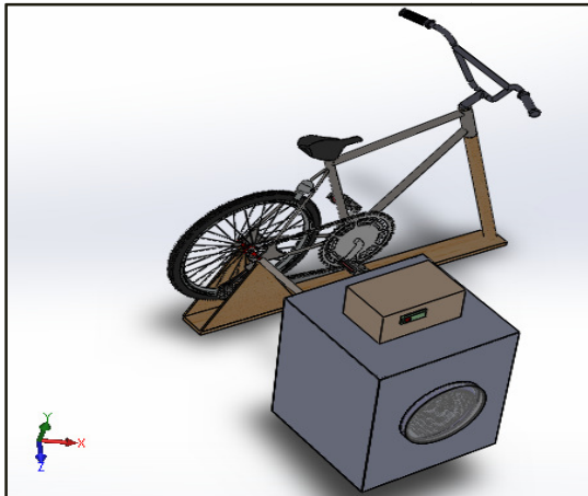
Figure 11. Assembled of the designed machine
