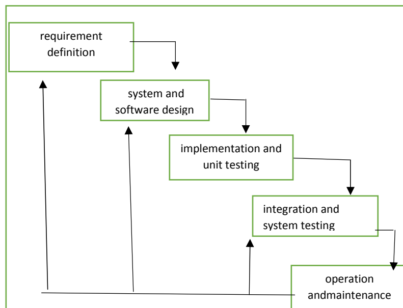
FIG.1: WATERFALL MODEL
